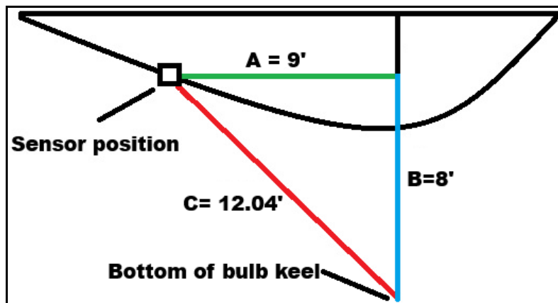
Figure 23: Sensor Position with Bulb Keel Overview
