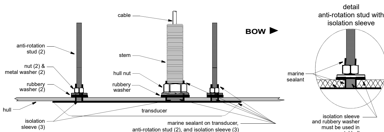
Figure 7. SS70, SS70-TS, SS141L: Bedding and installing WITHOUT a fairing in a metal hull (SS141L shown)
