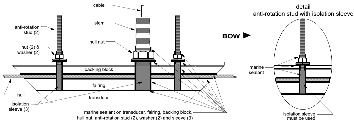
Figure 5. SS70, SS70-TS, SS141L: Bedding and installing with a fairing in a metal hull (SS141L shown)
