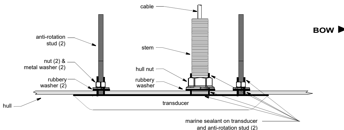
Figure 6. SS70, SS70-TS, SS141L: Bedding and installing WITHOUT a fairing in a fiberglass or wood hull (SS141L shown)
