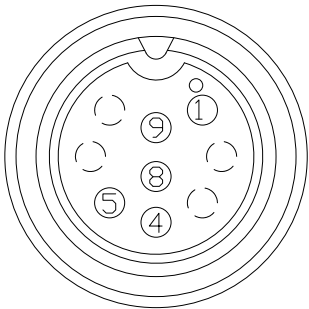
5/9 PIN MALE CONNECTOR
