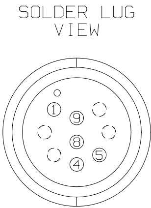
5/9 PIN MALE CONNECTOR
