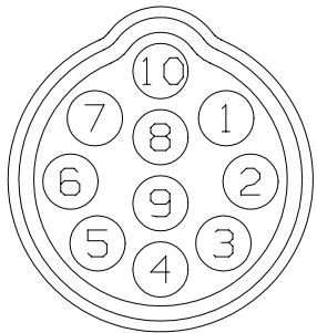
10 PIN MALE CONNECTOR
