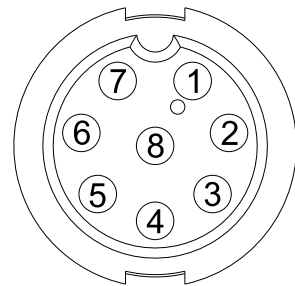
CONTACT END VIEW 8 PIN FEMALE GARMIN
