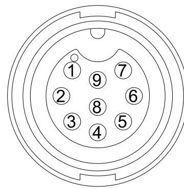
CONTACT END VIEW 9 PIN FEMALE
