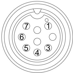
CONTACT END VIEW 6/9 PIN MALE
