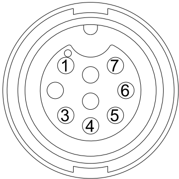
CONTACT END VIEW 6/9 PIN FEMALE
