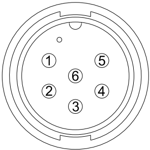
CONTACT END VIEW 6 PIN MALE
