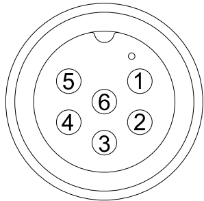
CONTACT END VIEW 6 PIN FEMALE
