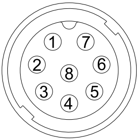
CONTACT END VIEW 8 PIN MALE
