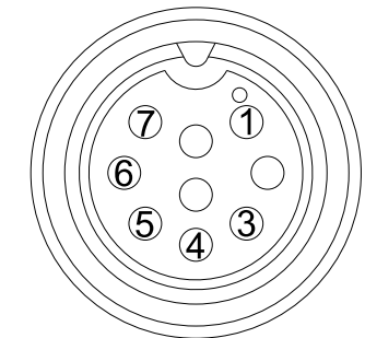
CONTACT END VIEW 6/9 PIN MALE
