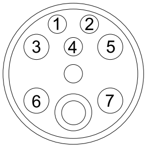
CONTACT END VIEW 7 PIN MALE
