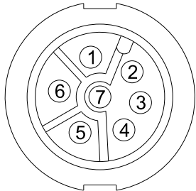
CONTACT END VIEW 7 PIN MALE
