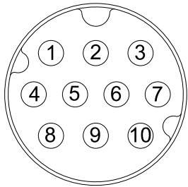
CONTACT END VIEW 10 PIN MALE
