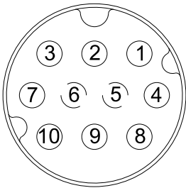
CONTACT END VIEW 8/10 PIN FEMALE
