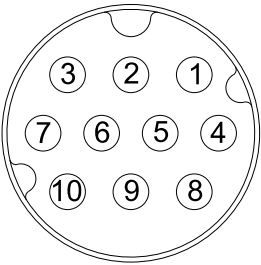
CONTACT END VIEW 10 PIN FEMALE
