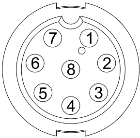
CONTACT END VIEW 8 PIN FEMALE GARMIN
