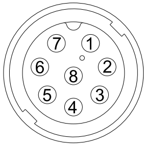
CONTACT END VIEW 8 PIN FEMALE
