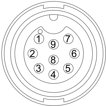
CONTACT END VIEW 9 PIN FEMALE
