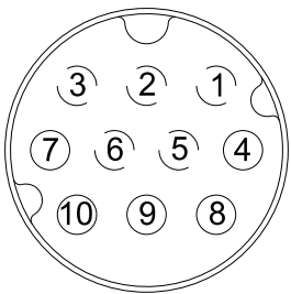
CONTACT END VIEW 5/10 PIN FEMALE
