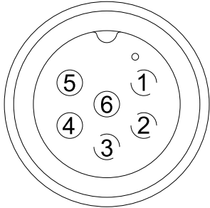
CONTACT END VIEW 3/6 PIN FEMALE
