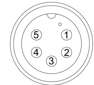
CONTACT END VIEW 5 PIN FEMALE
