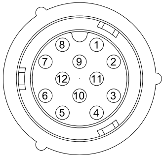
CONTACT END VIEW 12 PIN FEMALE
