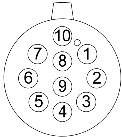
CONTACT END VIEW 10 PIN FEMALE
