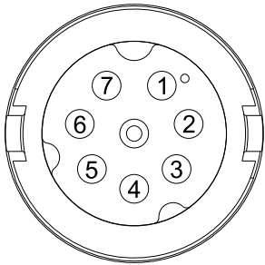
CONTACT END VIEW 7 PIN FEMALE
