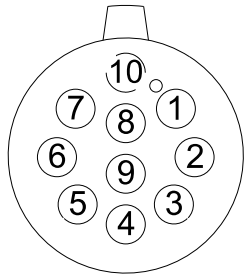
CONTACT END VIEW 9/10 PIN FEMALE
