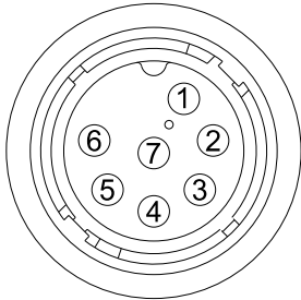
CONTACT END VIEW 7/8 PIN FEMALE
