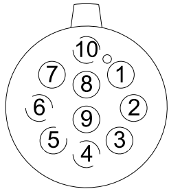
CONTACT END VIEW 6/10 PIN FEMALE
