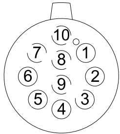
CONTACT END VIEW 5/10 PIN FEMALE
