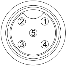
CONTACT END VIEW DEVICE NET
