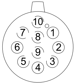
CONTACT END VIEW 4/10 PIN FEMALE
