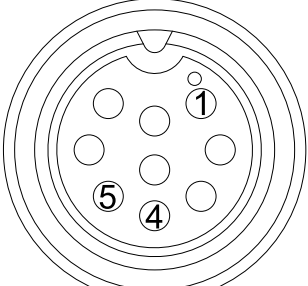
CONTACT END VIEW 3/9 PIN MALE
