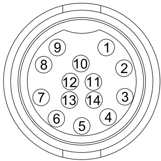
CONTACT END VIEW 14 PIN MALE
