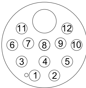
CONTACT END VIEW 12 PIN FEMALE
