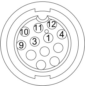
CONTACT END VIEW 7/12 FEMALE GARMIN
