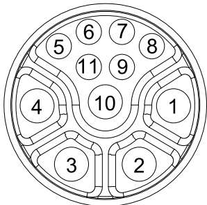
CONTACT END VIEW 11 PIN FEMALE
