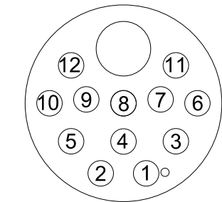
CONTACT END VIEW 12 PIN MALE
