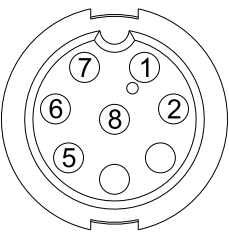
CONTACT END VIEW 6/8 FEMALE GARMIN
