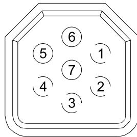
CONTACT END VIEW 3/7 MALE JOHNSON OUTDOORS
