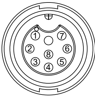
CONTACT END VIEW 8 PIN FEMALE
