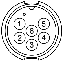
CONTACT END VIEW 6 PIN MALE
