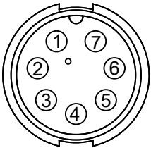
CONTACT END VIEW 7 PIN MALE
