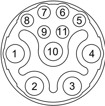
CONTACT END VIEW 11 PIN MALE
