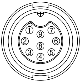
CONTACT END VIEW 9 PIN FEMALE
