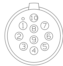
10 PIN MALE AIRMAR CONNECTOR
