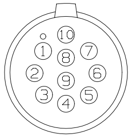
10 PIN MALE AIRMAR CONNECTOR
