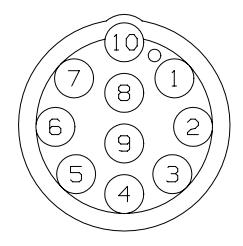
10 PIN MALE AIRMAR CONNECTOR
